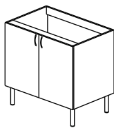
900 Base cabinet 900W x 580D x 865H Ref: OLBWC9
